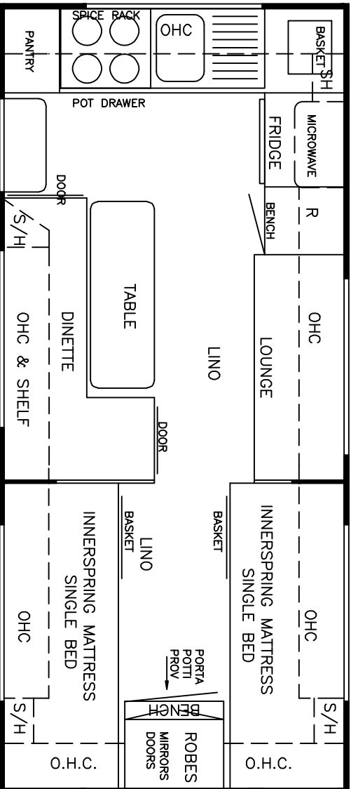
17' x 7' 9" - FDSB
