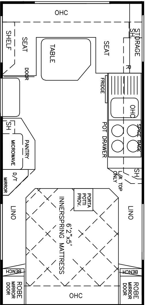
16'X7'9" - CLUB DB
