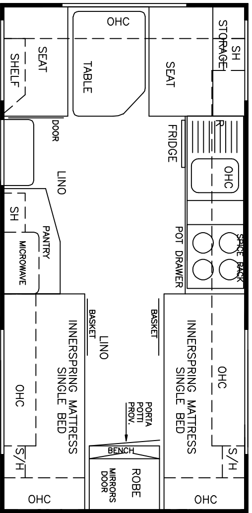
15'6" x 7'9" - CAFFFSB
