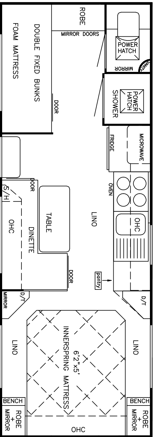
BELMONT LTD 21'6"X7'9"-9
