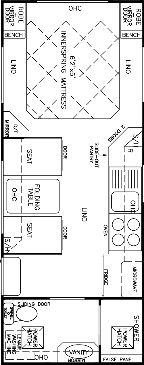
BELMONT LTD 19'x7'9" - 2CAFWD
