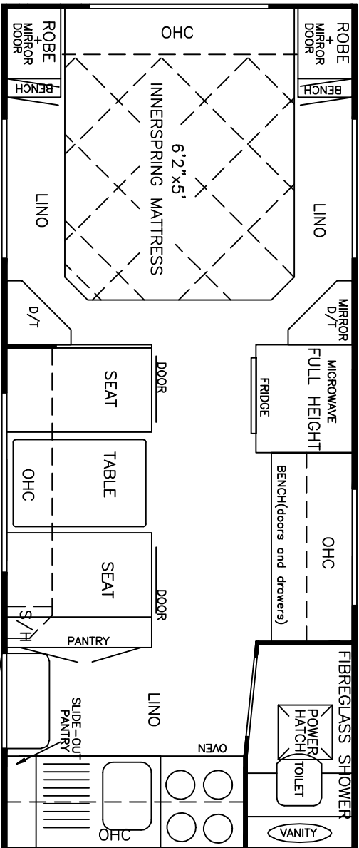
BELMONT LTD 18' x 7'9" -1
